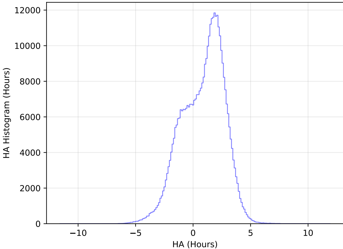
baseline_v2.1_10yrs All sky z band: HA Histogram
