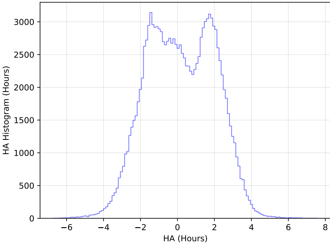
baseline_v2.1_10yrs All sky u band: HA Histogram
