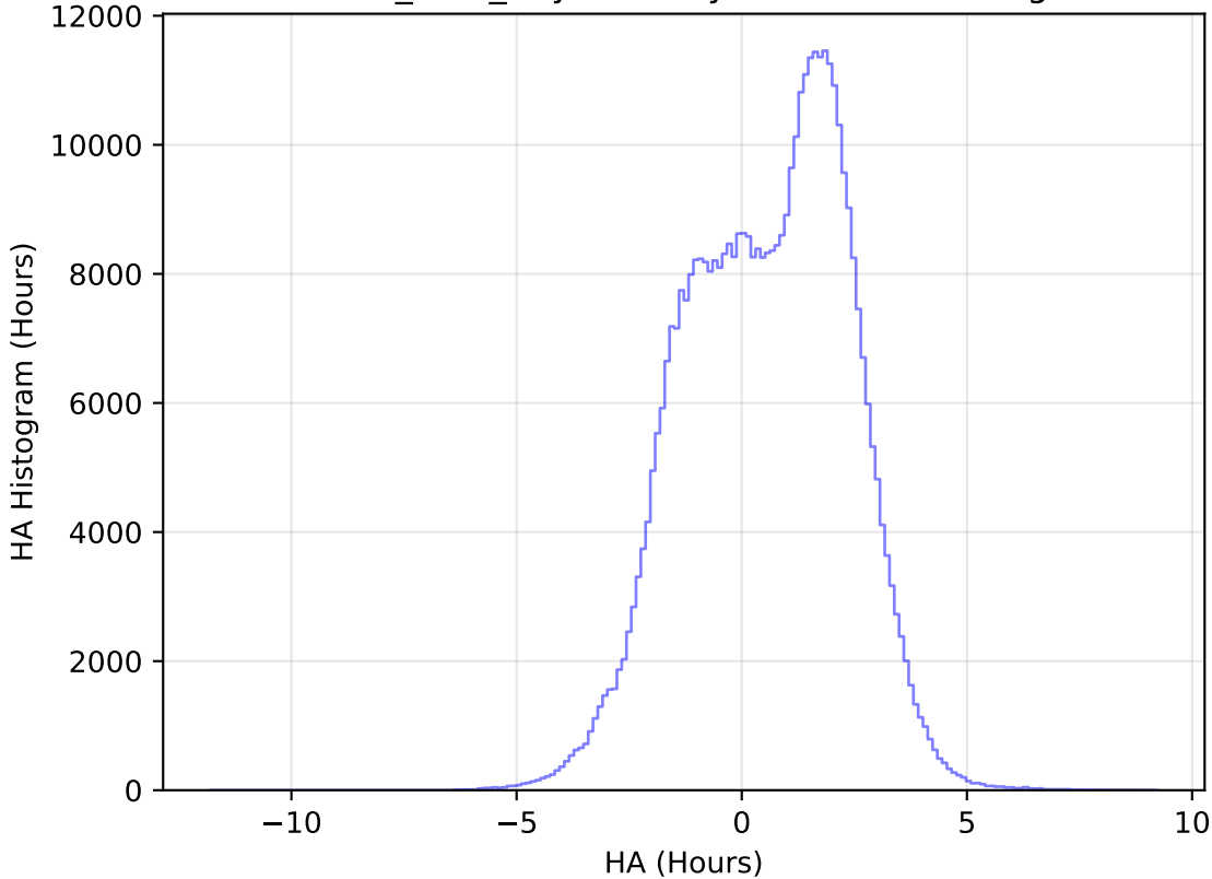
baseline_v2.1_10yrs All sky r band: HA Histogram
