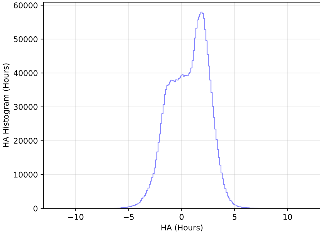
baseline_v2.1_10yrs All sky all bands: HA Histogram
