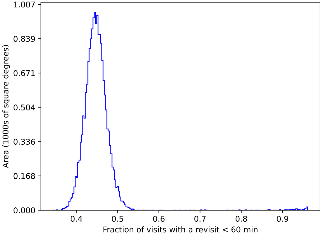
baseline_v2.1_10yrs gri WFD: Fraction of visits with a revisit < 60 min
