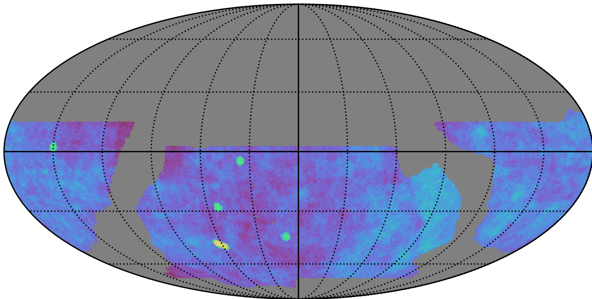
baseline_v2.1_10yrs gri WFD: Fraction of visits in pairs (20-90 min)
