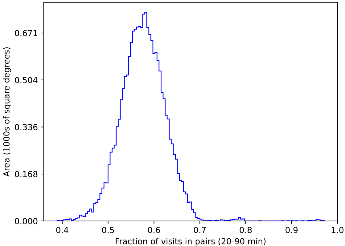
baseline_v2.1_10yrs gri WFD: Fraction of visits in pairs (20-90 min)
