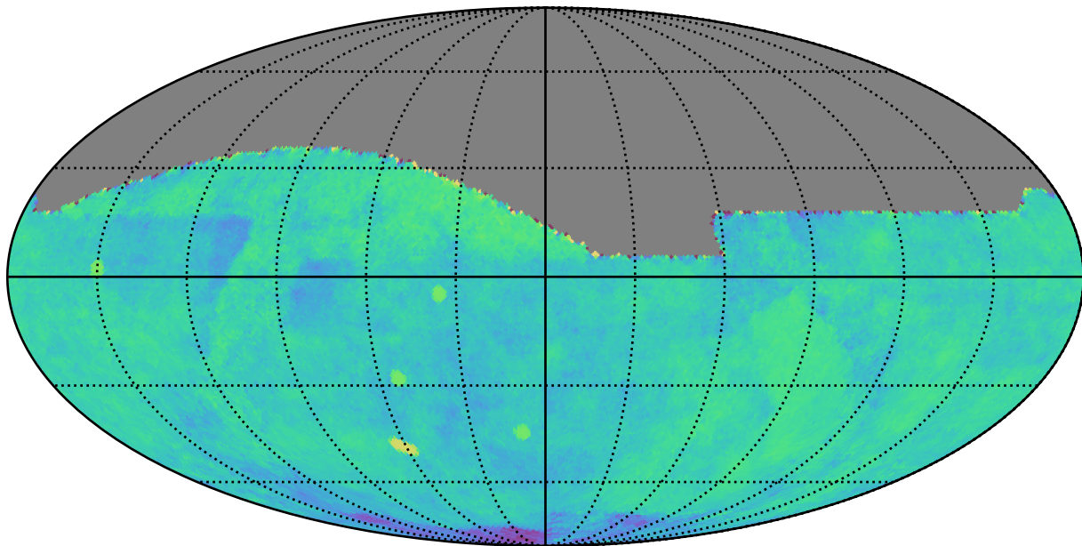
baseline_v2.1_10yrs gri All sky: Fraction of visits in pairs (20-90 min)
