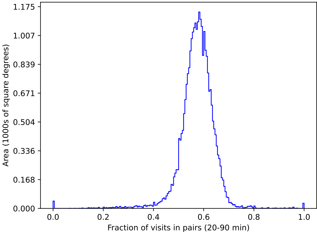
baseline_v2.1_10yrs gri All sky: Fraction of visits in pairs (20-90 min)
