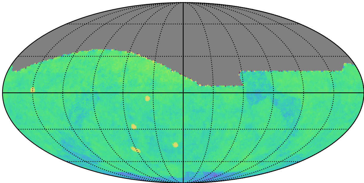
baseline_v2.1_10yrs gri All sky: Fraction of visits in pairs (10-60 min)
