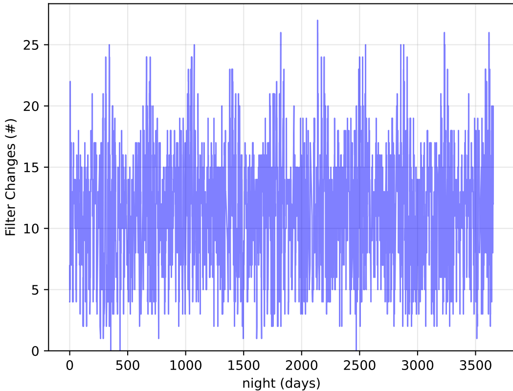
baseline_v2.1_10yrs Per Night: Filter Changes
