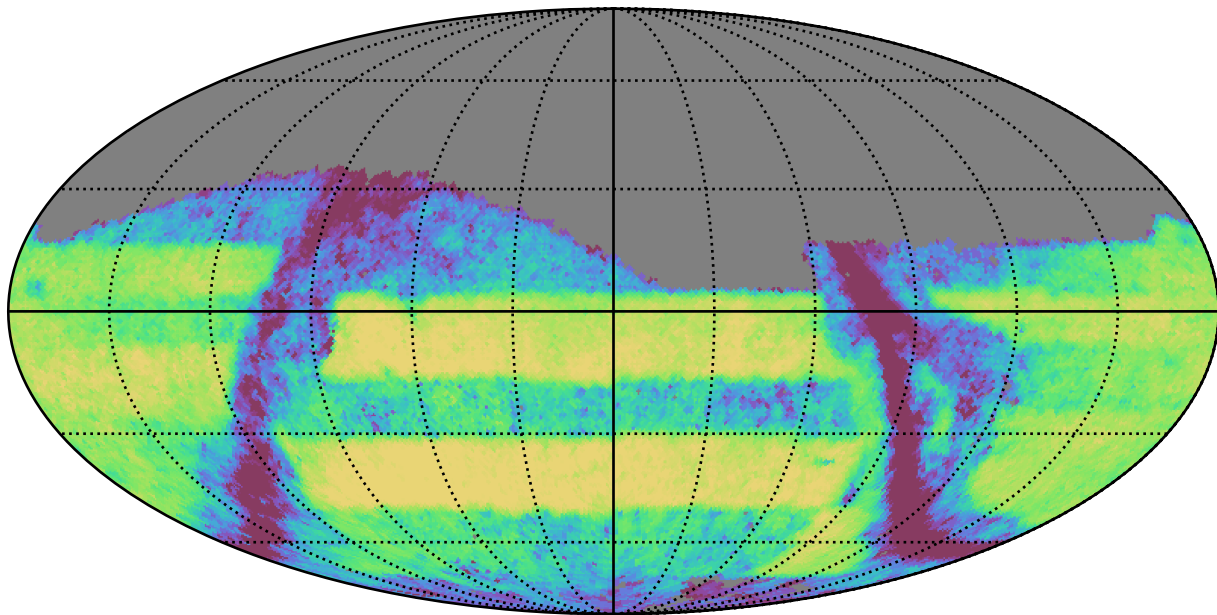
baseline_v2.1_10yrs Yr 3-4 z band: Exgal_CoaddM5
