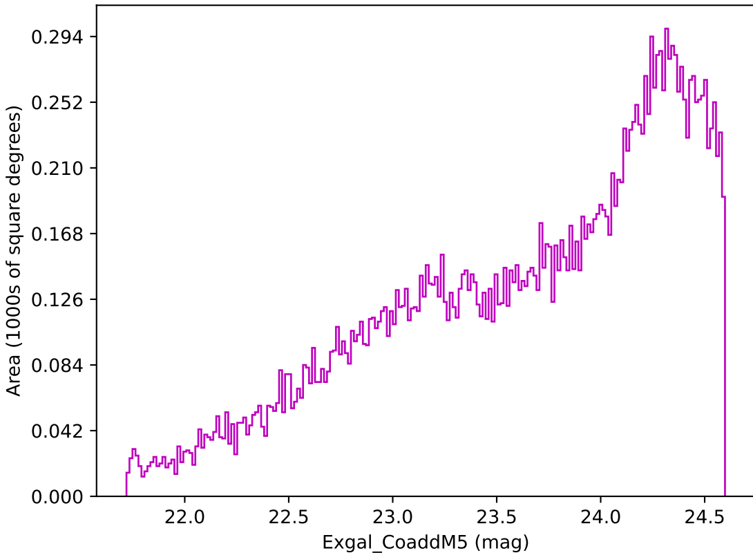
baseline_v2.1_10yrs Yr 3-4 z band: Exgal_CoaddM5
