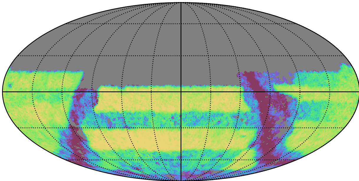
baseline_v2.1_10yrs Yr 3-4 y band: Exgal_CoaddM5
