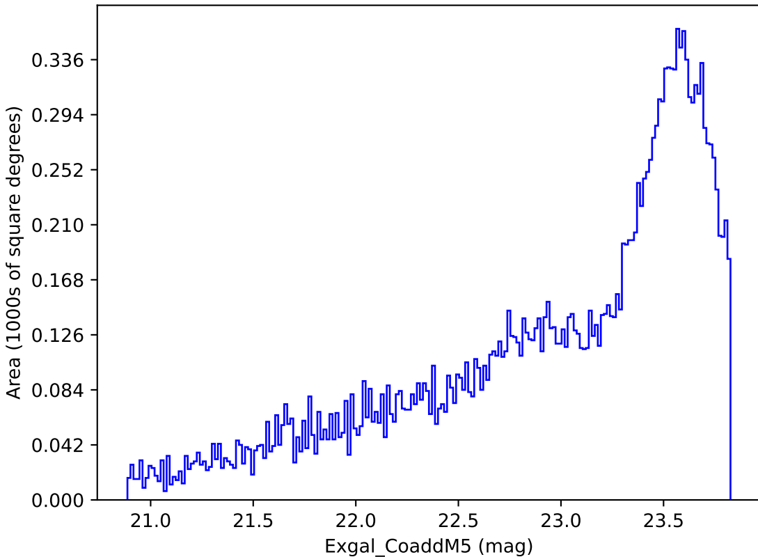
baseline_v2.1_10yrs Yr 3-4 y band: Exgal_CoaddM5
