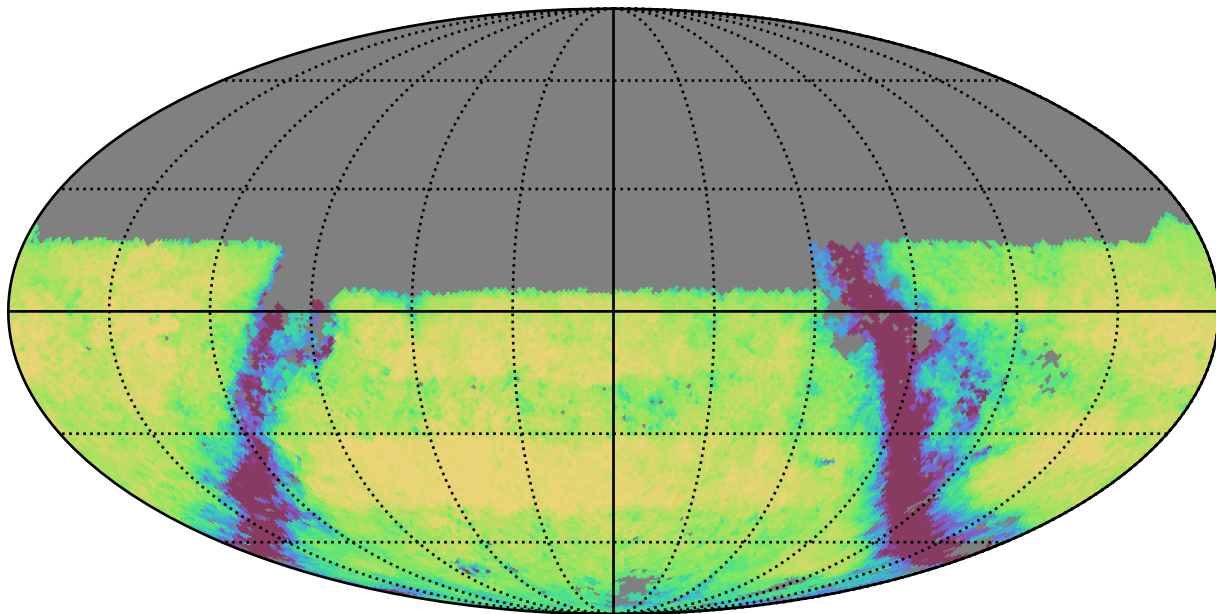
baseline_v2.1_10yrs Yr 3-4 u band: Exgal_CoaddM5
