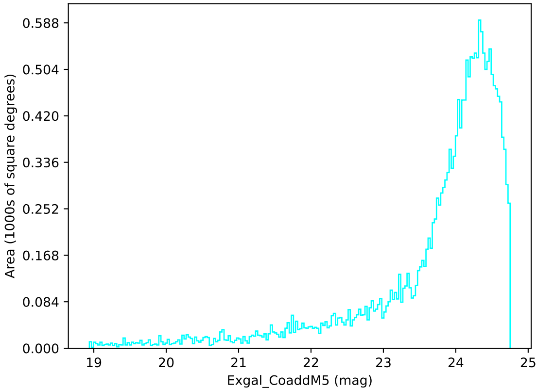
baseline_v2.1_10yrs Yr 3-4 u band: Exgal_CoaddM5
