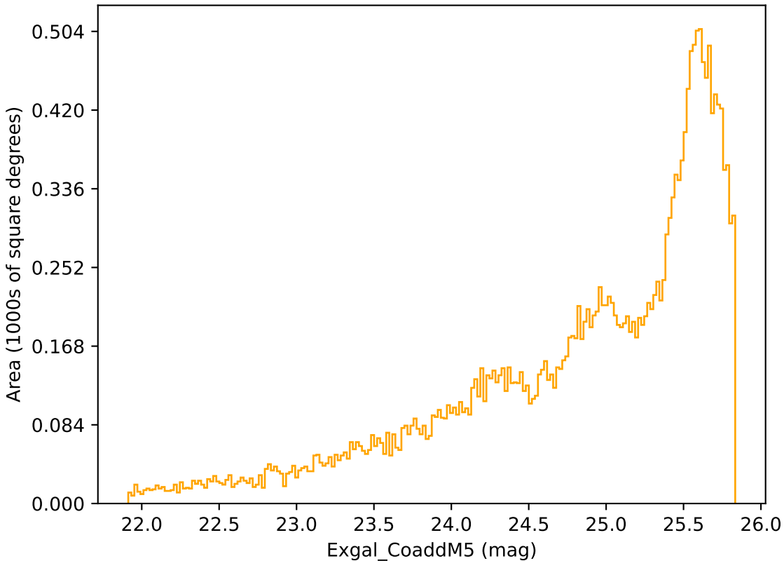
baseline_v2.1_10yrs Yr 3-4 r band: Exgal_CoaddM5
