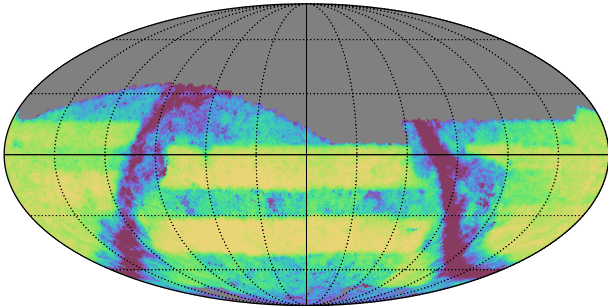
baseline_v2.1_10yrs Yr 3-4 i band: Exgal_CoaddM5
