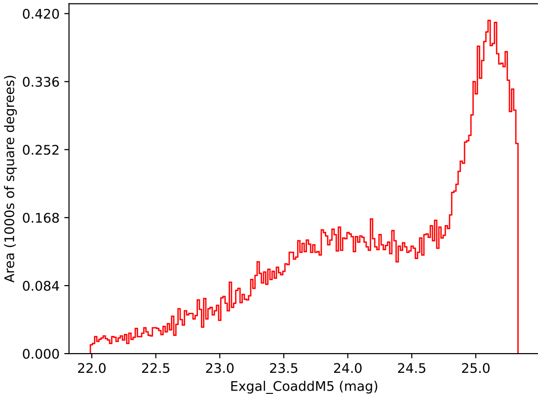
baseline_v2.1_10yrs Yr 3-4 i band: Exgal_CoaddM5
