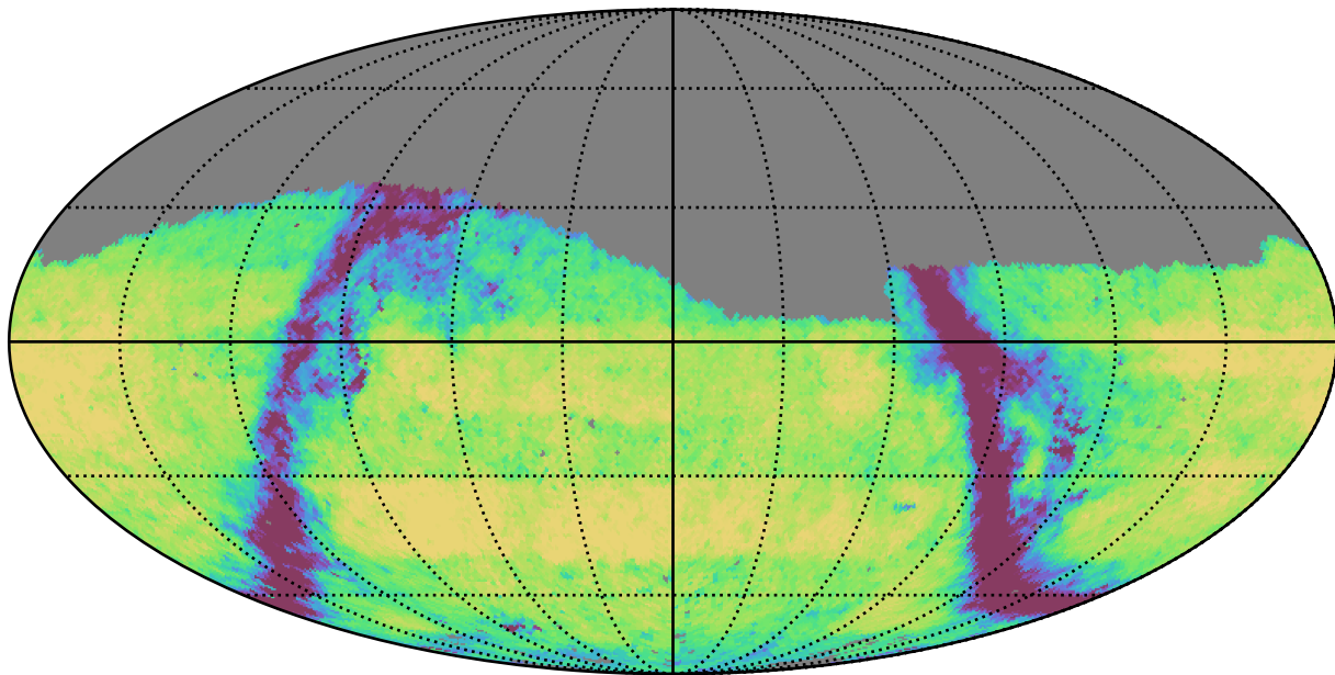
baseline_v2.1_10yrs Yr 3-4 g band: Exgal_CoaddM5
