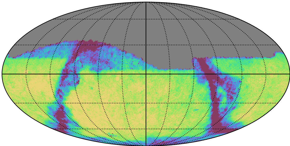
baseline_v2.1_10yrs Yr 1 z band: Exgal_CoaddM5
