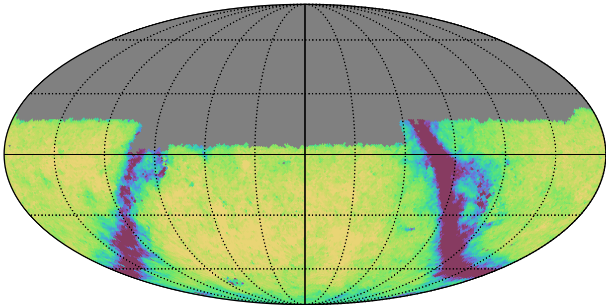
baseline_v2.1_10yrs Yr 1 u band: Exgal_CoaddM5
