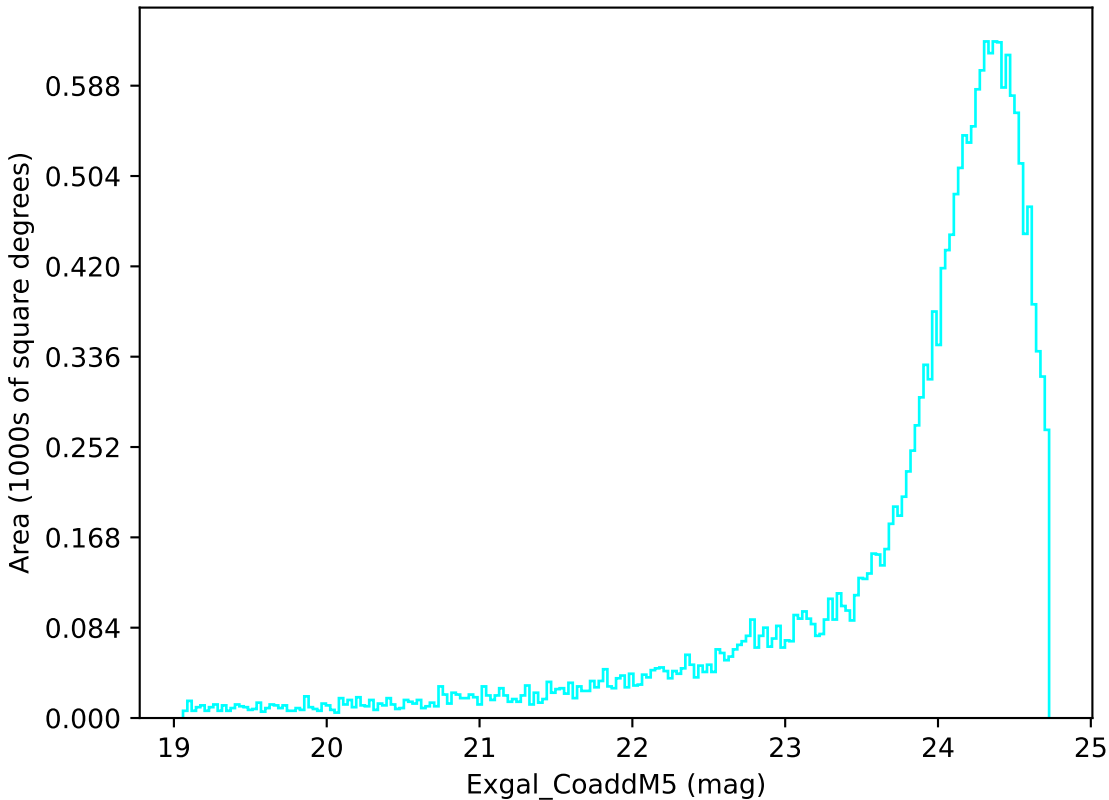
baseline_v2.1_10yrs Yr 1 u band: Exgal_CoaddM5
