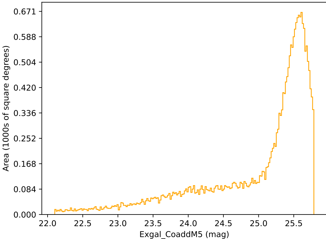
baseline_v2.1_10yrs Yr 1 r band: Exgal_CoaddM5
