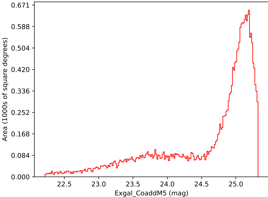
baseline_v2.1_10yrs Yr 1 i band: Exgal_CoaddM5
