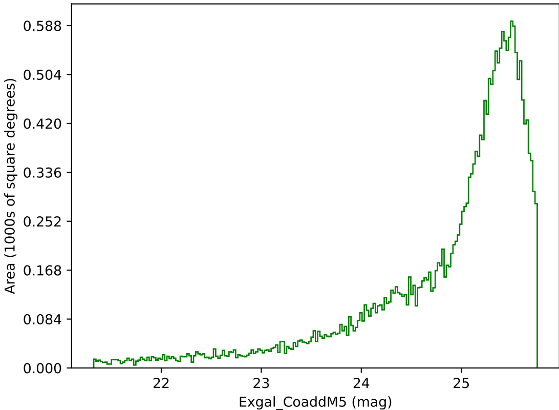
baseline_v2.1_10yrs Yr 1 g band: Exgal_CoaddM5
