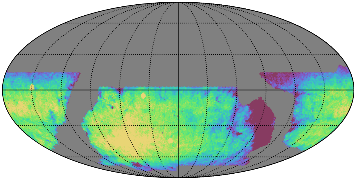
baseline_v2.1_10yrs WFD z band: Exgal_CoaddM5
