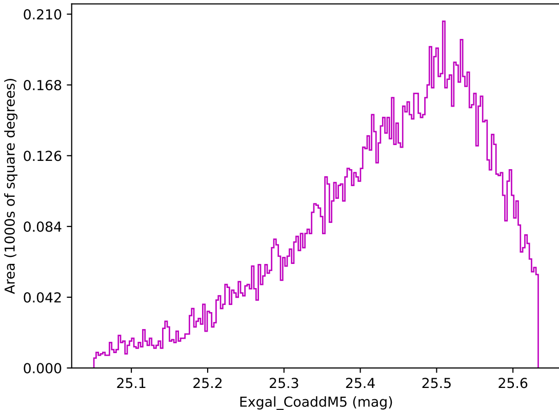
baseline_v2.1_10yrs WFD z band: Exgal_CoaddM5
