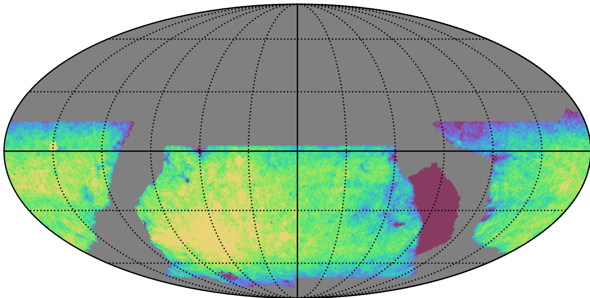
baseline_v2.1_10yrs WFD y band: Exgal_CoaddM5
