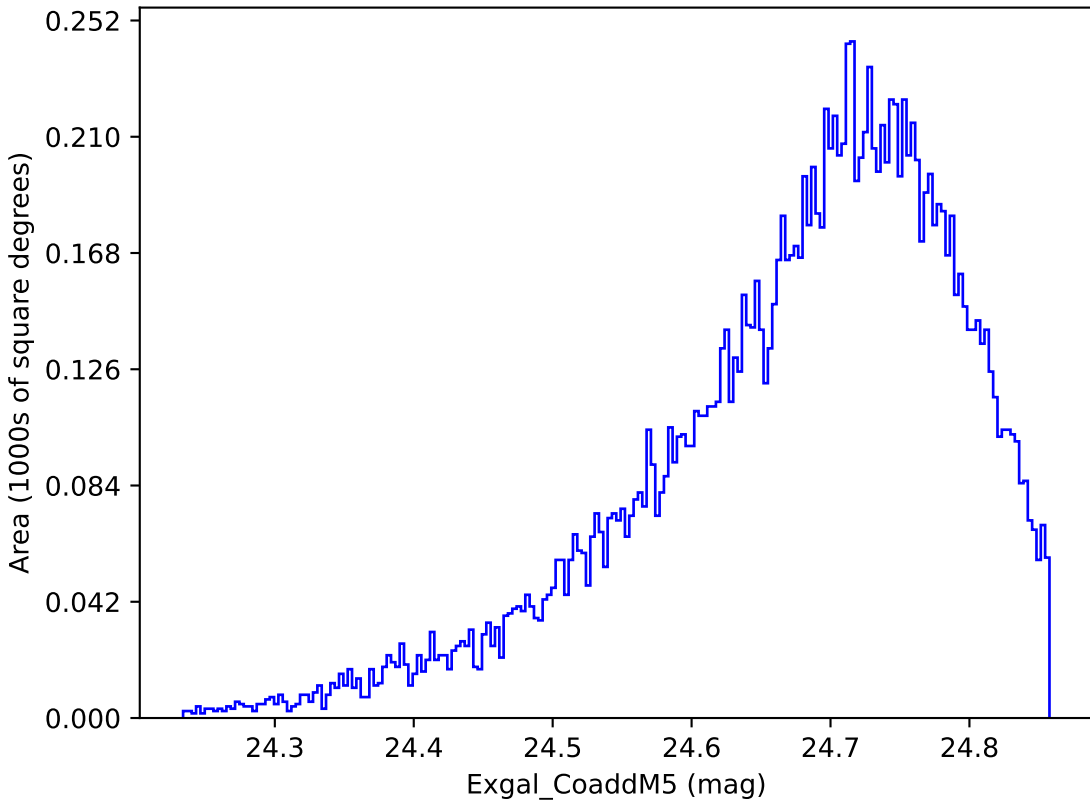
baseline_v2.1_10yrs WFD y band: Exgal_CoaddM5
