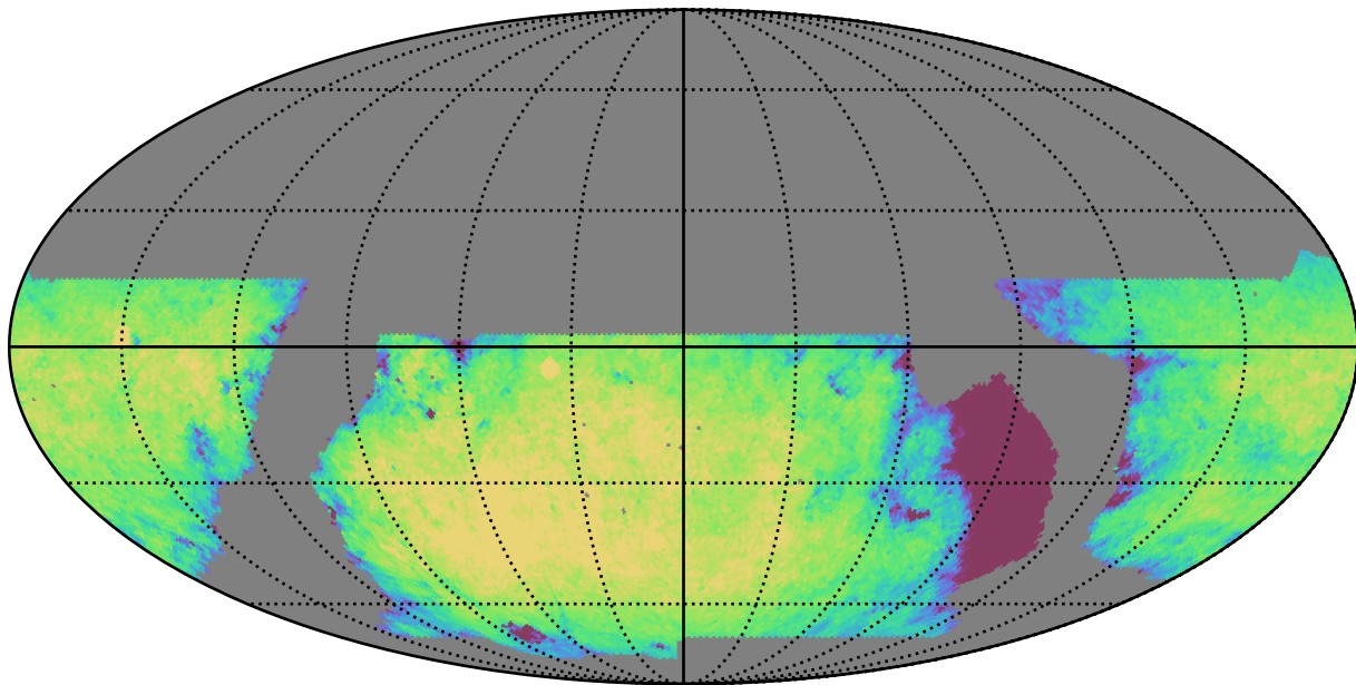
baseline_v2.1_10yrs WFD u band: Exgal_CoaddM5
