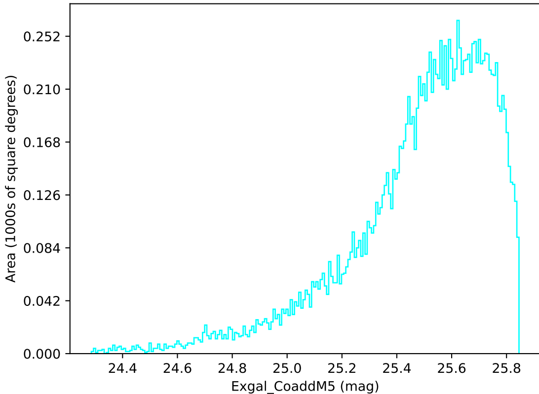
baseline_v2.1_10yrs WFD u band: Exgal_CoaddM5
