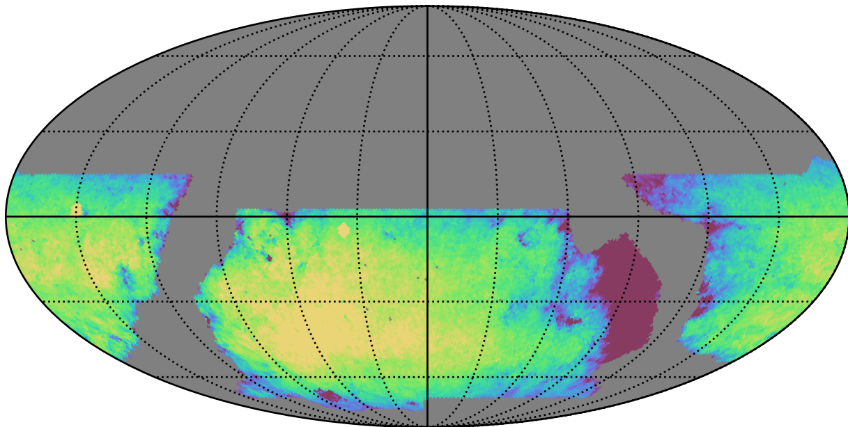
baseline_v2.1_10yrs WFD r band: Exgal_CoaddM5
