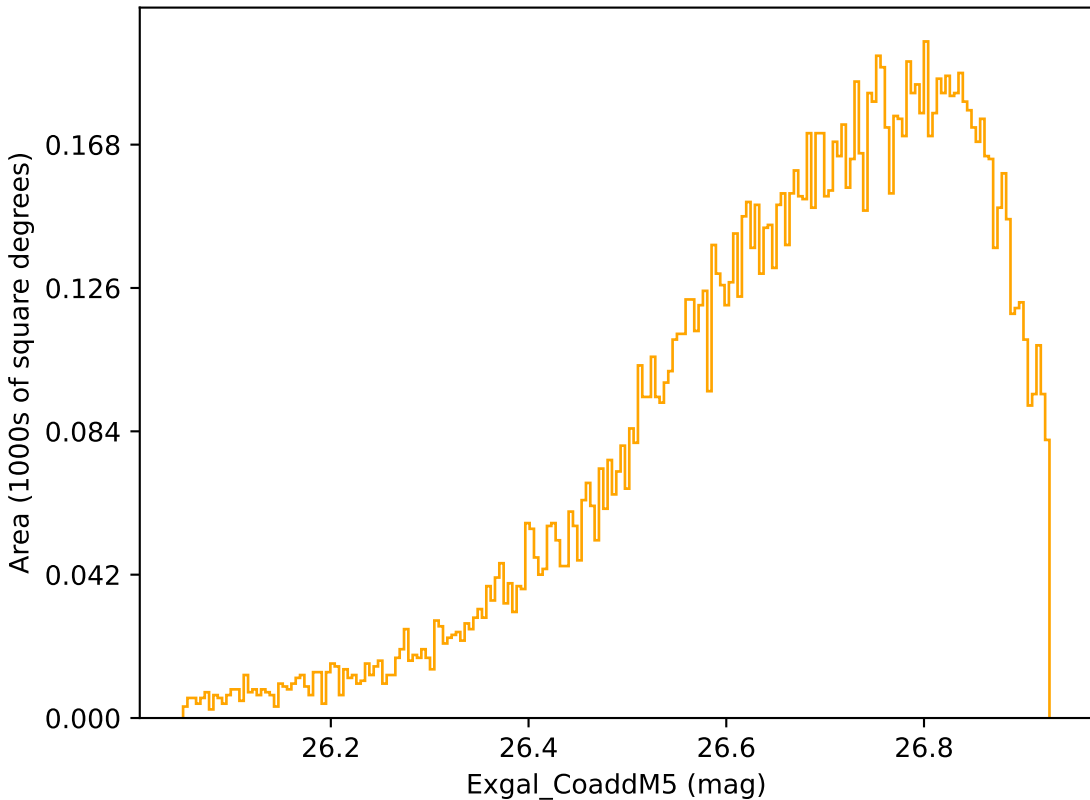
baseline_v2.1_10yrs WFD r band: Exgal_CoaddM5
