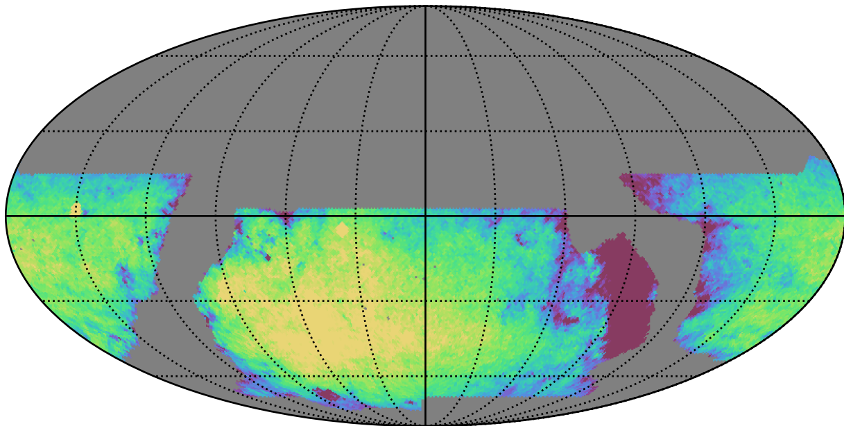
baseline_v2.1_10yrs WFD g band: Exgal_CoaddM5
