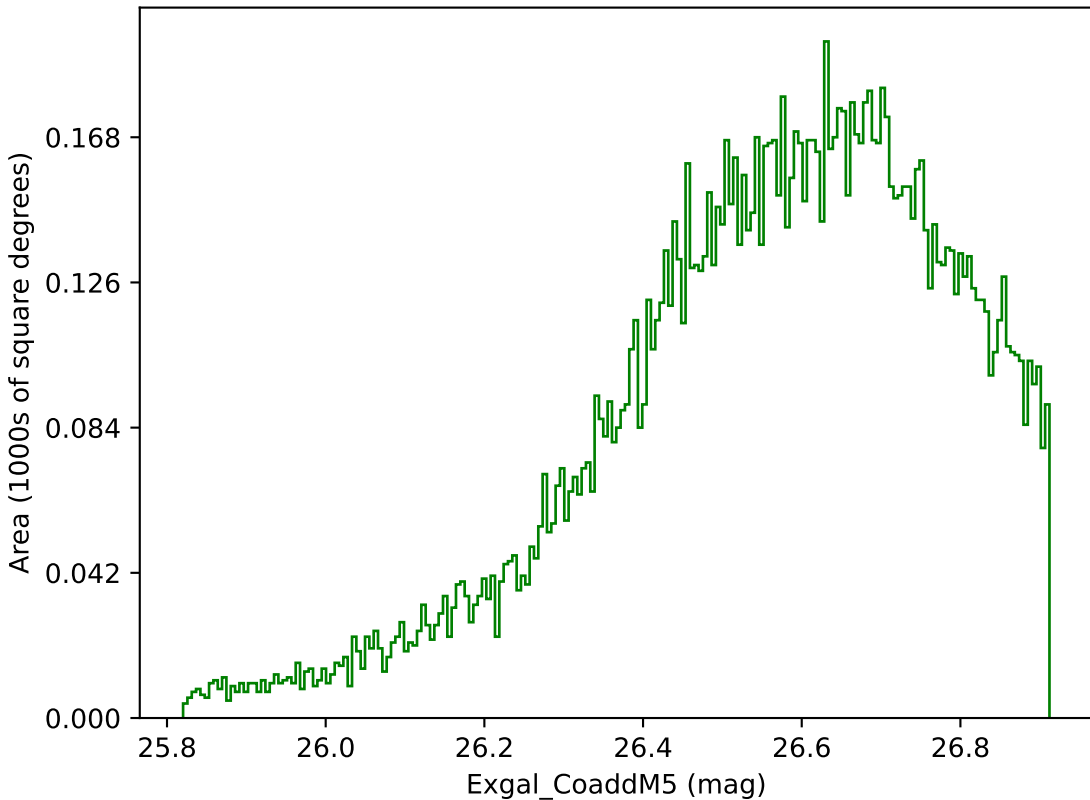
baseline_v2.1_10yrs WFD g band: Exgal_CoaddM5
