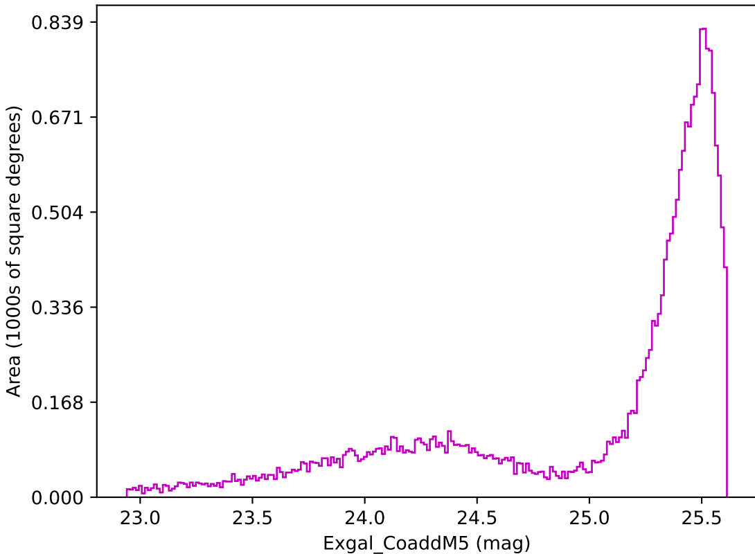
baseline_v2.1_10yrs All sky z band: Exgal_CoaddM5
