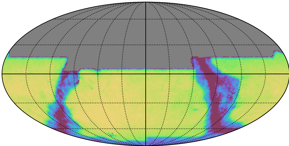
baseline_v2.1_10yrs All sky y band: Exgal_CoaddM5
