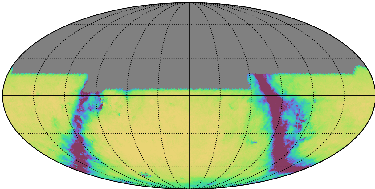
baseline_v2.1_10yrs All sky u band: Exgal_CoaddM5
