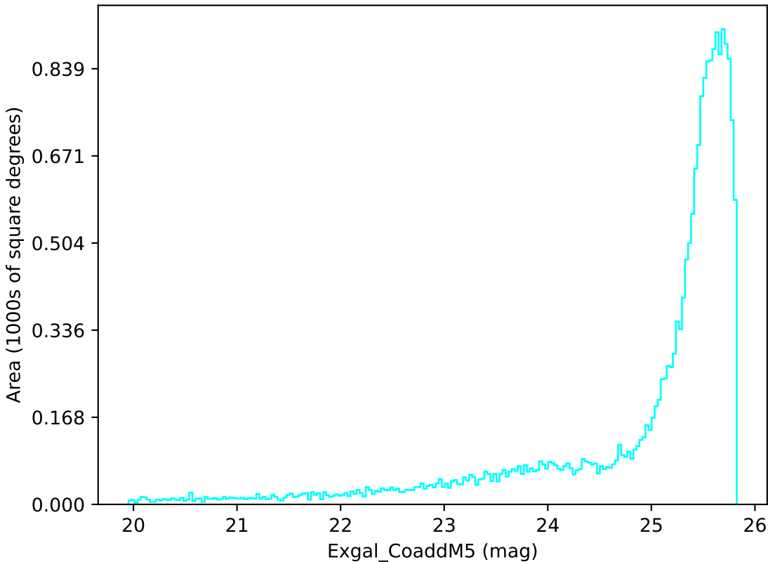
baseline_v2.1_10yrs All sky u band: Exgal_CoaddM5
