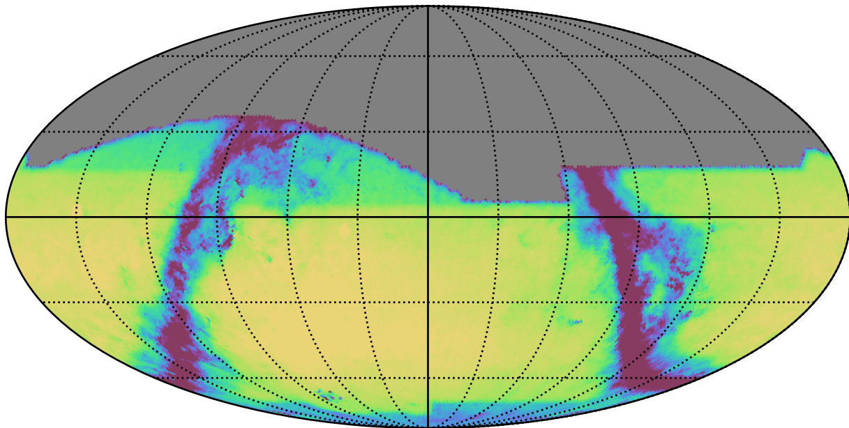
baseline_v2.1_10yrs All sky r band: Exgal_CoaddM5
