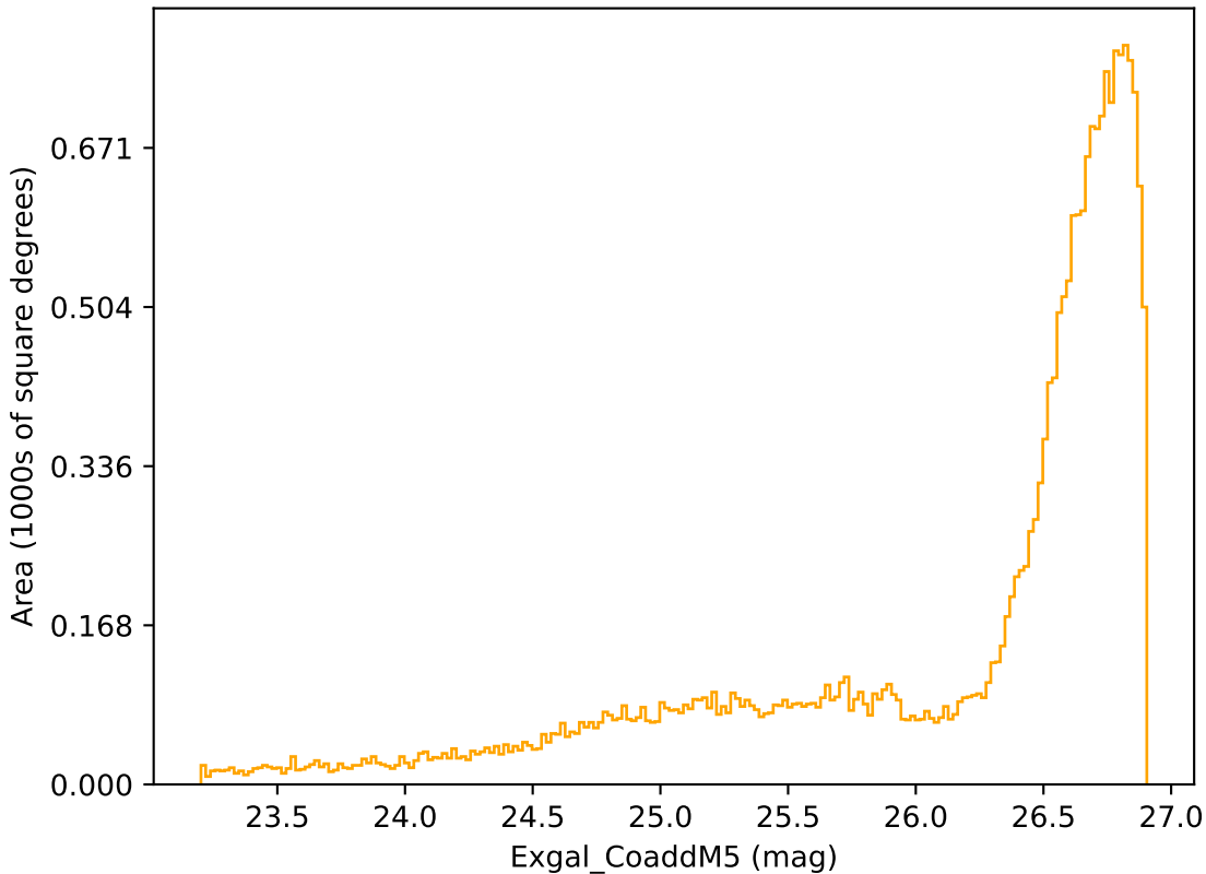
baseline_v2.1_10yrs All sky r band: Exgal_CoaddM5
