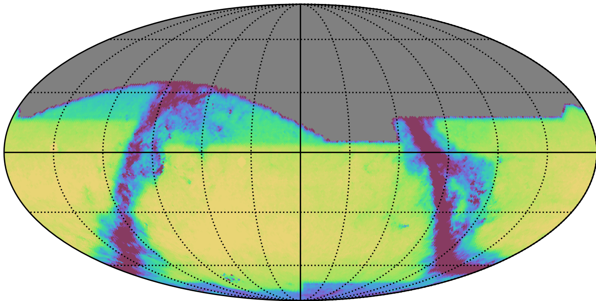
baseline_v2.1_10yrs All sky i band: Exgal_CoaddM5
