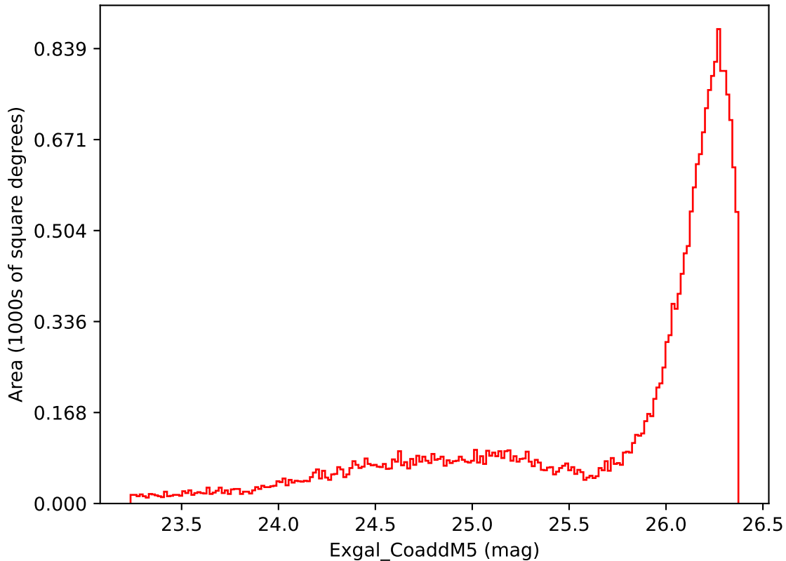
baseline_v2.1_10yrs All sky i band: Exgal_CoaddM5
