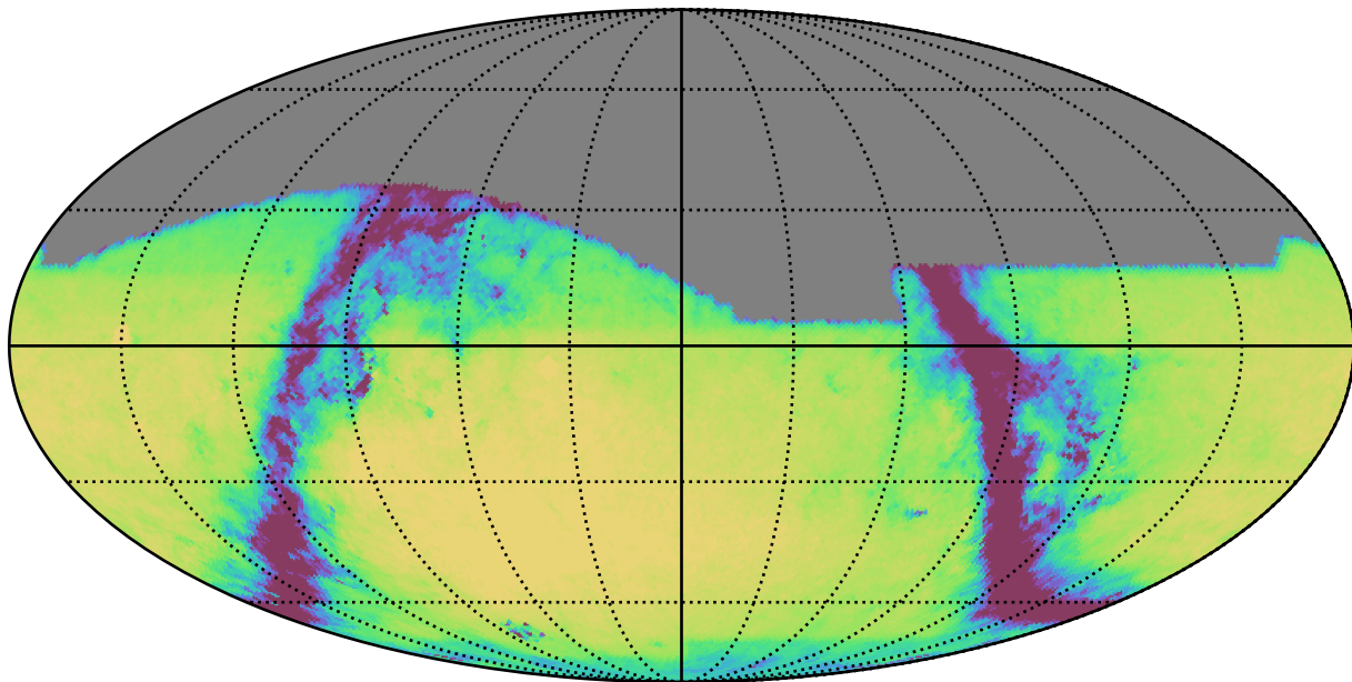
baseline_v2.1_10yrs All sky g band: Exgal_CoaddM5
