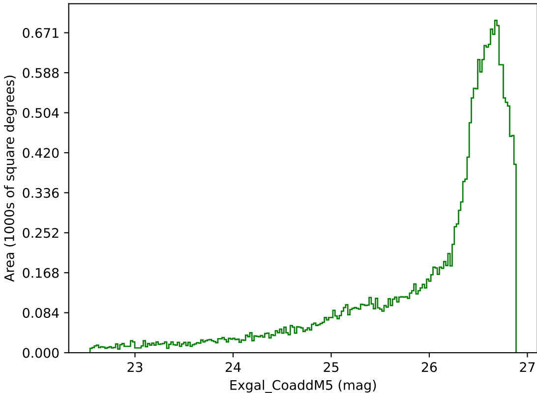
baseline_v2.1_10yrs All sky g band: Exgal_CoaddM5
