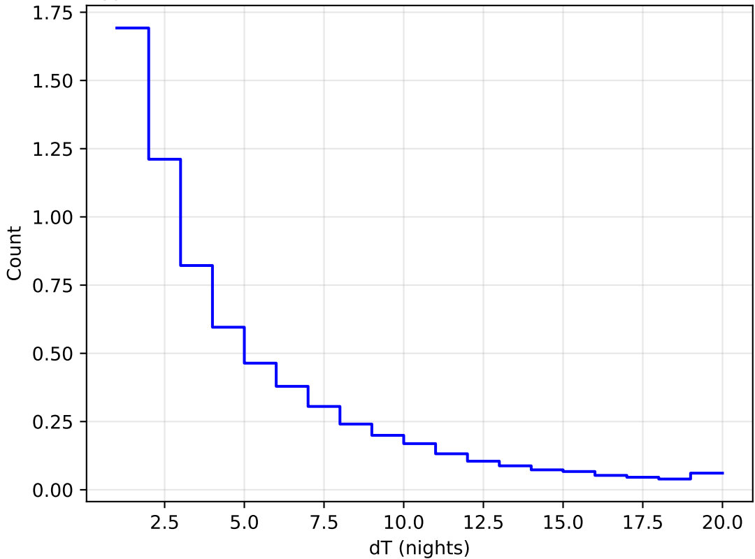
baseline_v2.1_10yrs WFD all bands: DeltaNight Histogram 1e6
