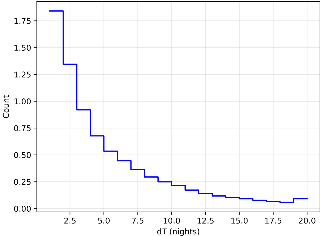
baseline_v2.1_10yrs All sky all bands: DeltaNight Histogram 1e6
