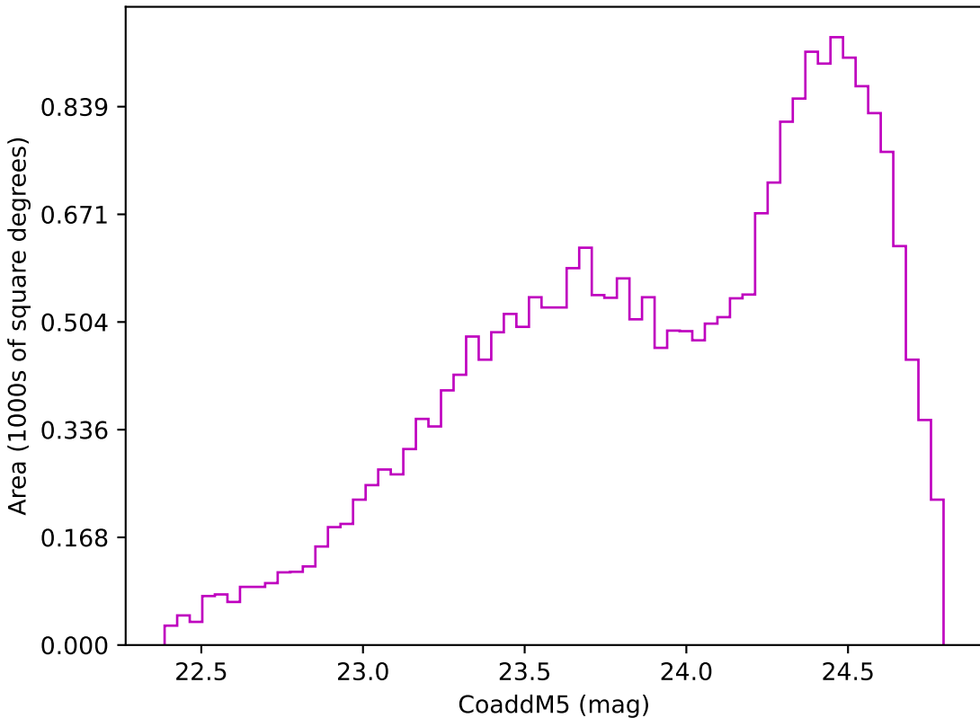
baseline_v2.1_10yrs Yr 3-4 z band: CoaddM5
